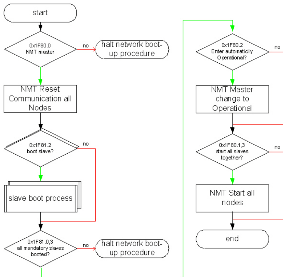
Figure 3-3 CANopen Boot-up Procedure – Main Flow
