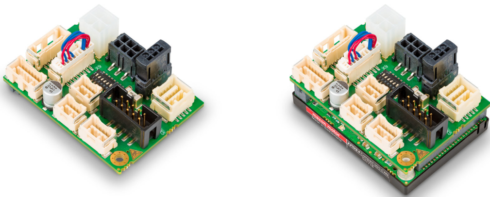
図 3-12 EPOS4 CB 50/5 CAN (左) / EPOS4 Compact 50/5 CAN (右)
