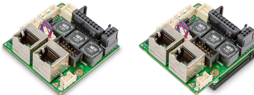
図 3-13 EPOS4 CB 24/1.5 EtherCAT (左) / EPOS4 Compact 24/1.5 EtherCAT (右)
