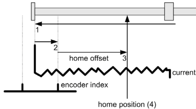
Figure 5-19 Homing Method -2
